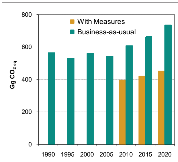
Figure 4-6 Greenhouse gas emissions in the “Waste” sector in 1990-2005 and projections by 2020
