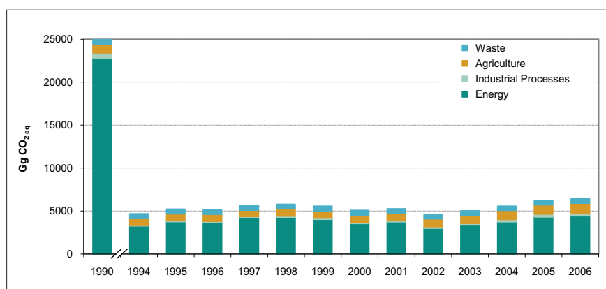
Figure 2-6 Greenhouse gas emissions by sectors, 1990-2006
