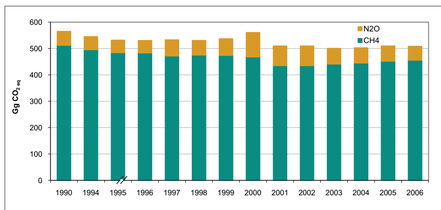
Figure 2-12 Greenhouse gas emissions by gases in the "Waste" sector, 1990-2006
