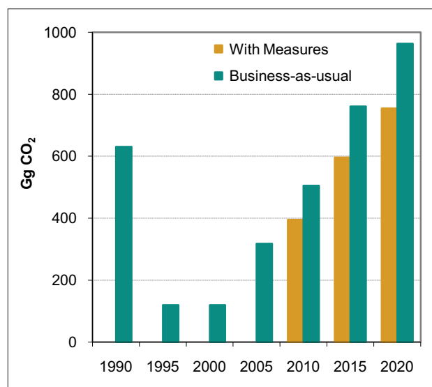
Figure 4-3 CO 2 emissions in the "Industrial Processes" sector in 1990-2005 and projections by 2020
