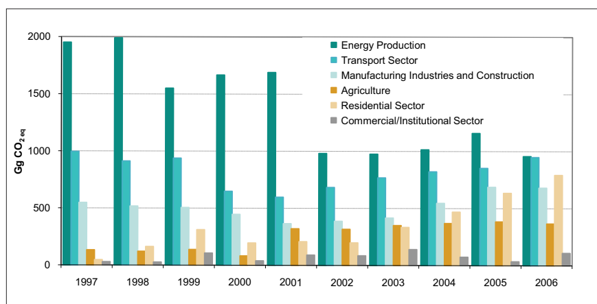
Figure 2-8 Greenhouse gas emissions from fuel combustion in the "Energy" sector, 1997-2006
