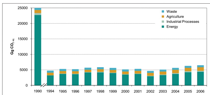
Figure ES-2 Greenhouse gas emissions by sectors, 1990-2006 (without LULUCF)
