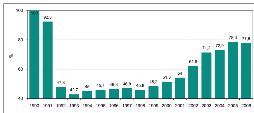
Figure 1-4 Dynamics of industrial production, 1990-2006
