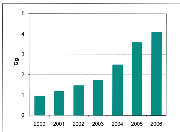
Figure 2-10 NMVOC emissions in the "Solvent Use" sector, 2000-2006
