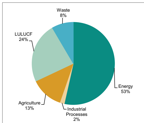
Figure 2-3 Distribution of greenhouse gas emissions by sectors, 2000 (CO 2 eq)
