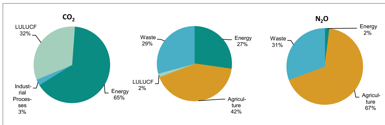
Figure 2-4 Distribution of greenhouse gas emissions in sectors by gases, 2000
