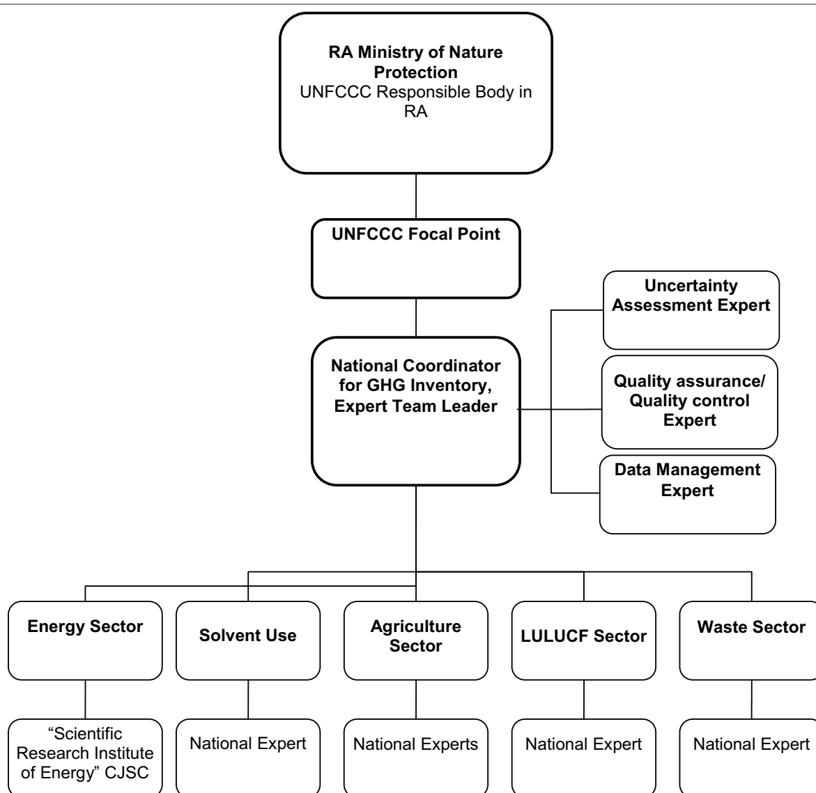
Figure 2.1 Organizational chart for preparation of the Second National Inventory of Greenhouse Gases
