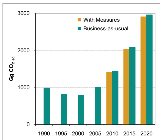
Figure 4-4 Greenhouse gas emissions in the "Agriculture" sector in 1990-2005 and projections by 2020
