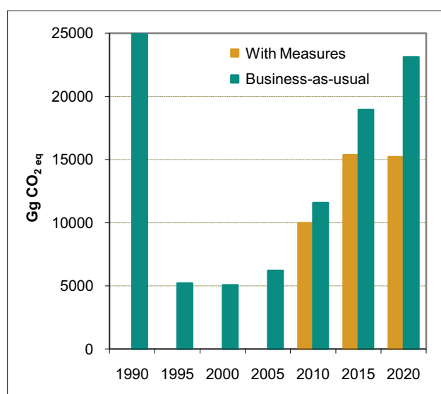
Figure 4-1 Total greenhouse gas emissions in 1990-2005 and projections by 2020
