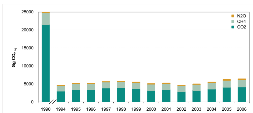
Figure ES-1 Greenhouse gas emissions by gases, 1990-2006 (without LULUCF)
