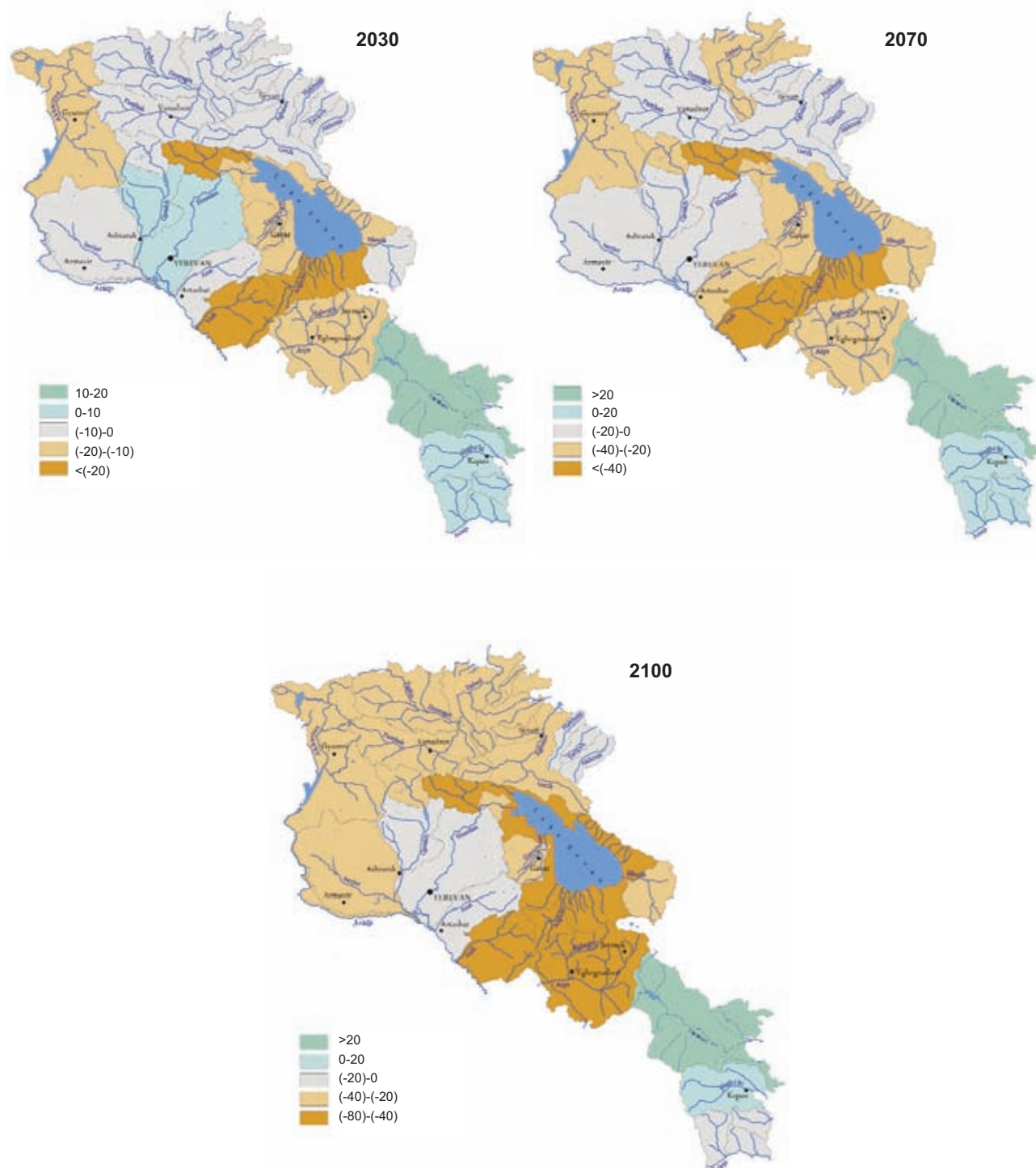
Figure 5-5 Forecasted changes in the river flow by river basins
