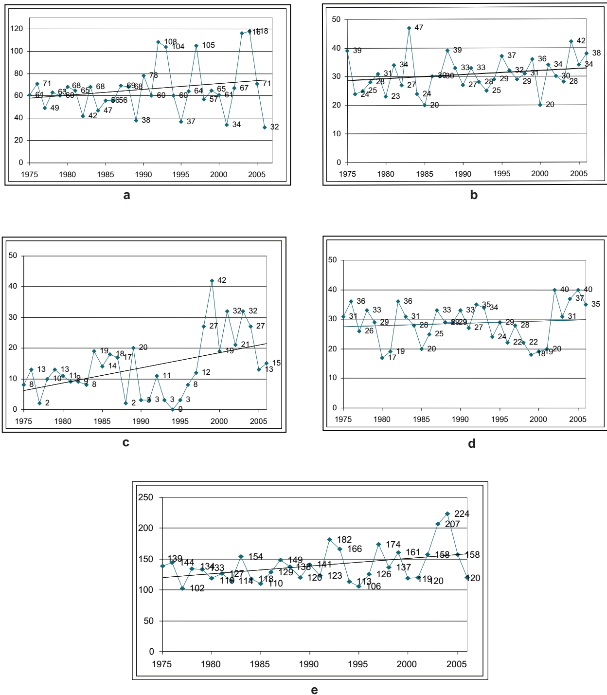
Figure 5-3 Number of extreme hydro-meteorological events in Armenia, 1975-2005 – frosts (a), hails (b), heavy rainfalls (c), strong winds (d), total (e)
