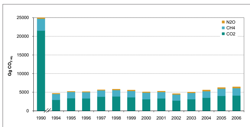
Figure 2-5 Greenhouse gas emissions by gases, 1990-2006
