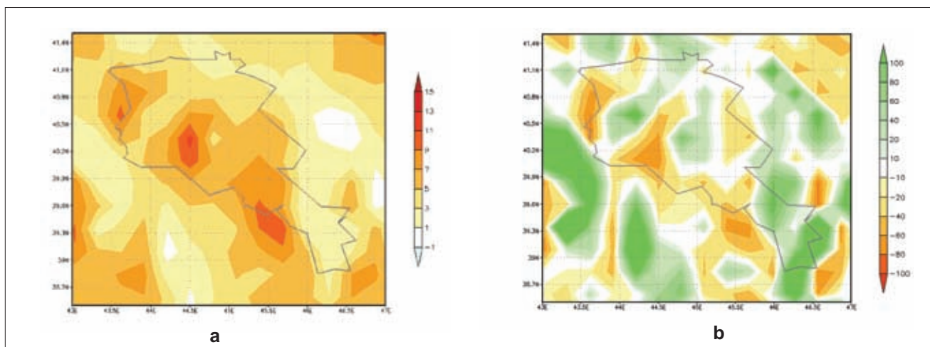
Figure 5-4 Annual (a) air temperature (°C) and (b) precipitation (%) changes in 2071-2100 compared to the average for 1961-1990, according to PRECIS model under A2 scenario of IPCC
