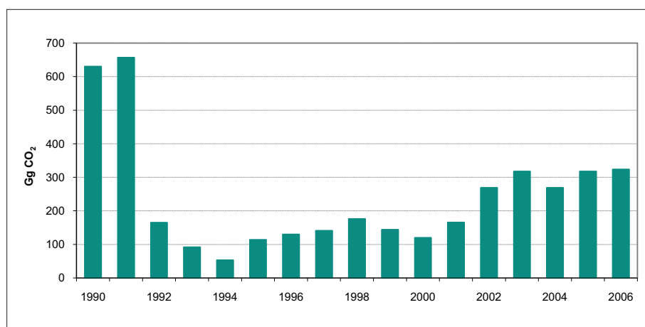
Figure 2-9 Greenhouse gas emissions in the "Industrial Processes" sector, 1990-2006
