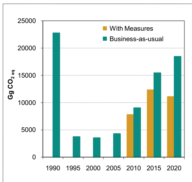
Figure 4-2 Greenhouse gas emissions in the “Energy” sector in 1995-2005 and projections by 2020
