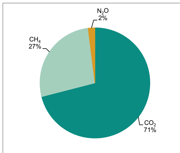
Figure 2-2 Distribution of greenhouse gas emissions by gases, 2000 (CO 2 eq)
