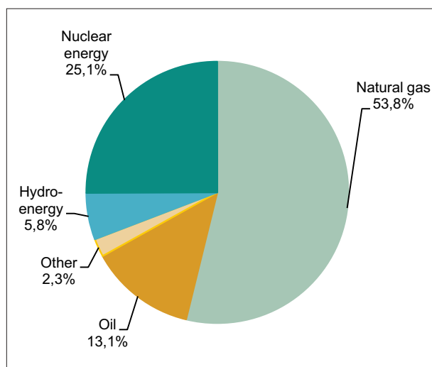
Figure 1-2 Proportion of energy sources in general energy consumption, 2006
