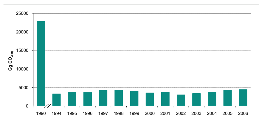
Figure 2-7 Greenhouse gas emissions in the "Energy" sector, 1990-2006
