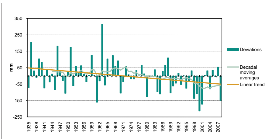
Figure 5-1 Deviations of average annual air temperature (a) and precipitation (b) from the average values for 1961-1990
